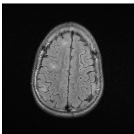
tuberous-sclerosis- cns- sclerosis- s lung
